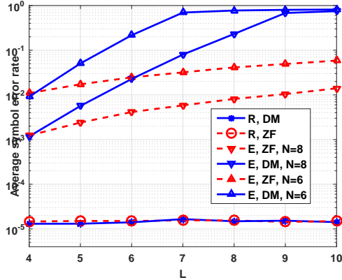
Fig. 3: Average SER versus the number of transmitting antennas for the directional modulation and the benchmark schemes when K = 4 , \sqrt{\gamma} = 8 , and \beta = 8 .
