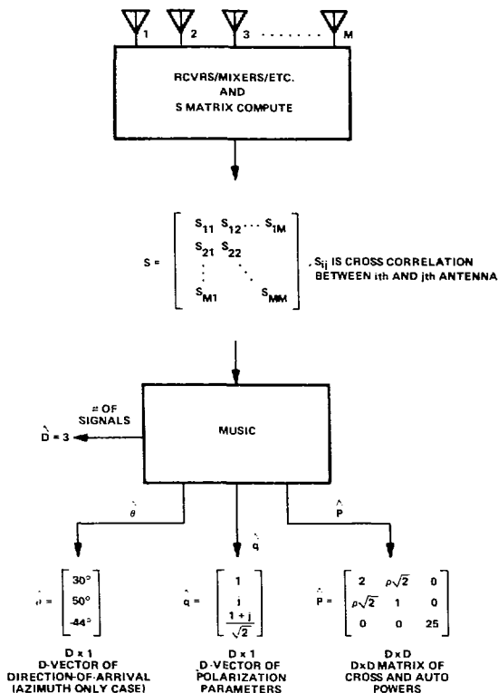
Fig. 2. Block diagram for multiple signal classification.
